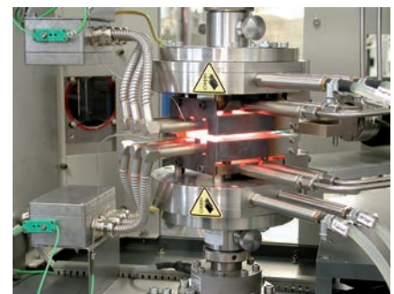
Fig. 3: Testing of catalytic converter mats
