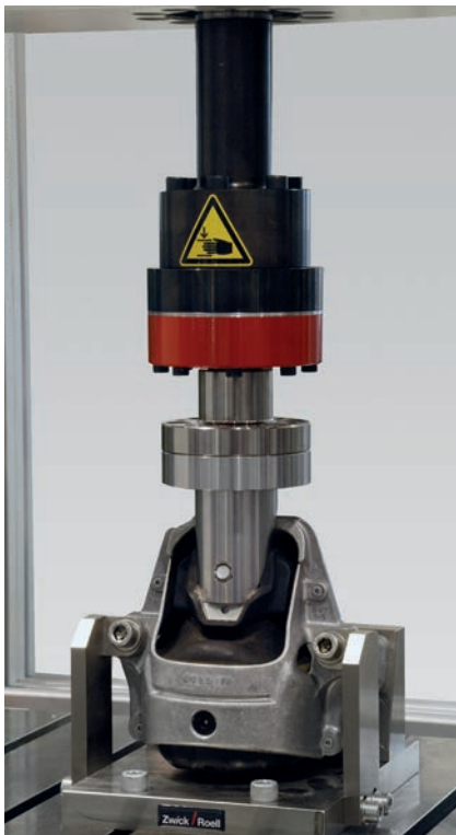
Fig. 1: Single-axis fatigue testing on engine mounts
