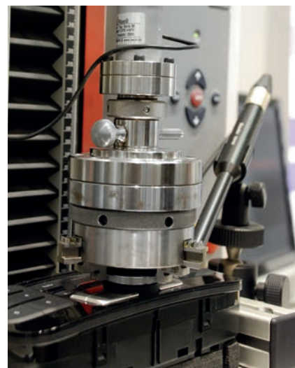
Fig. 3: Acoustic-haptic tests on multi-function rotary switches
