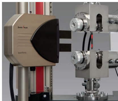
Fig. 3: Specimen grip and extensometer can be retrofitted at any time
