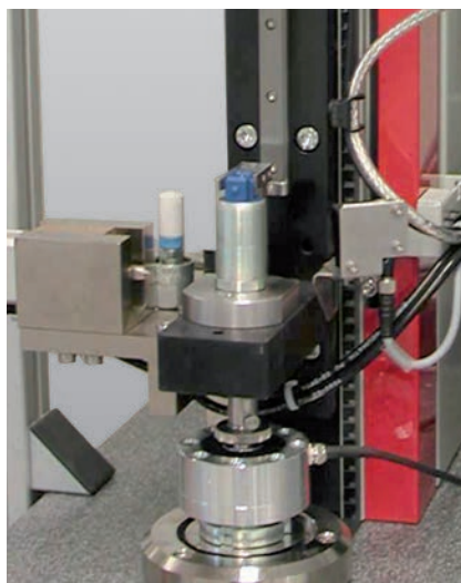
Fig. 1: Testing of electromagnetic actuators
