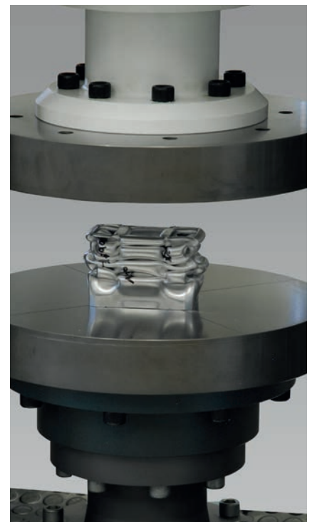
Fig. 1: AllroundLine materials testing machine with two test areas for tensile and compression tests on body components
