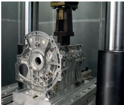
Fig. 1: Fatigue tests on the engine block
