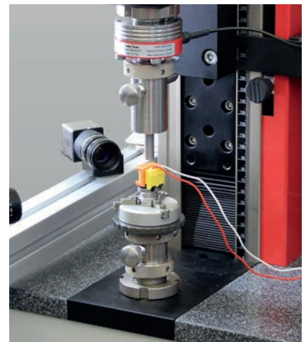
Fig. 3: Testing of airbag connectors
